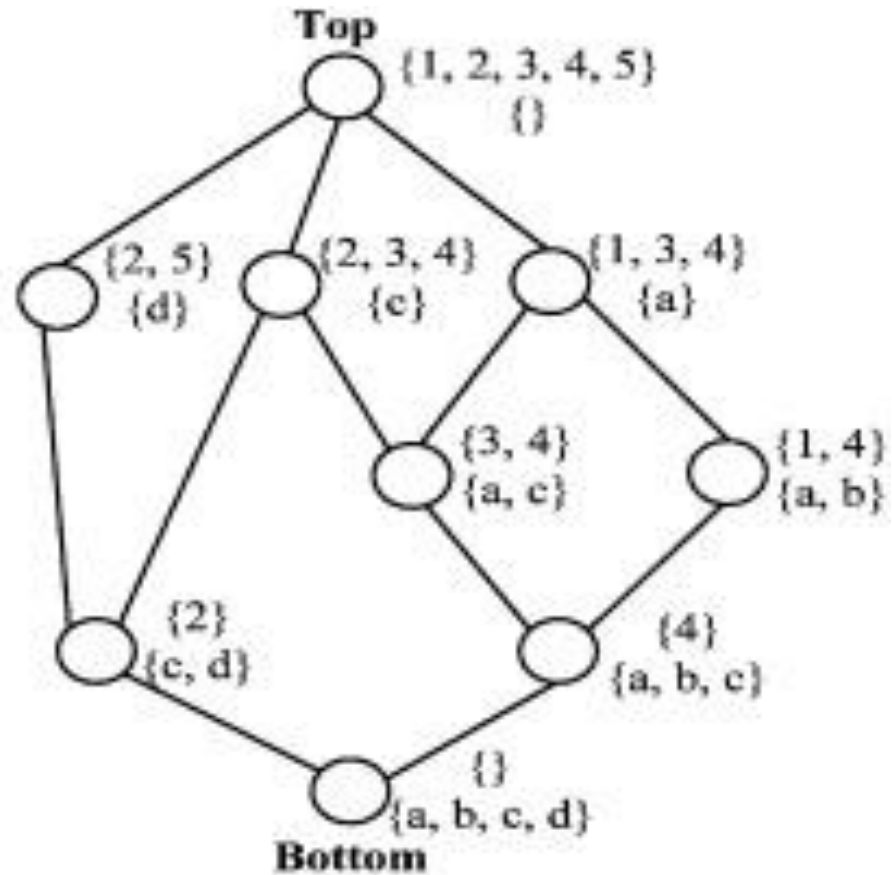
(b) Concept lattice
